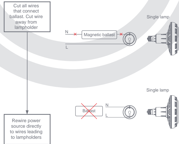
Diagram 3 – Magnetic ballast fixture wiring modification
