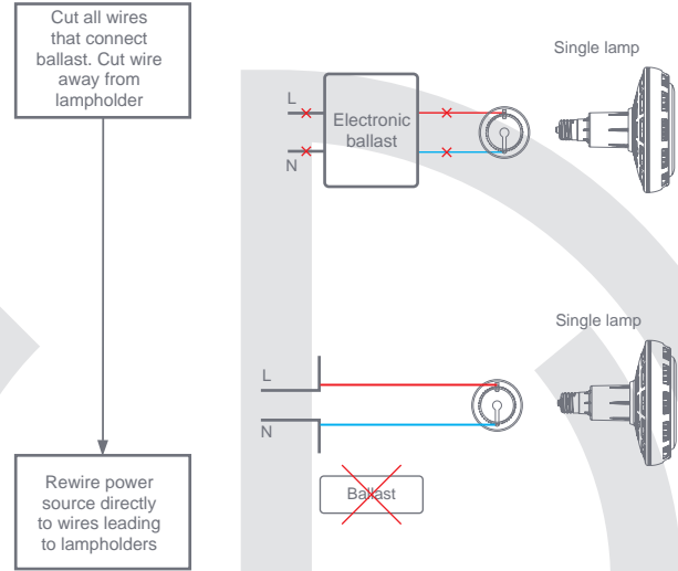
Diagram 2 – Electronic ballast fixture wiring modification
