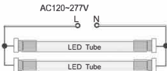
Double-Ended Bypass
