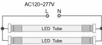
Double-Ended Bypass
