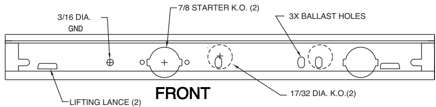
TOP WITHOUT DIFFUSER
