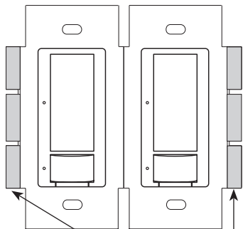
Each control has inside fins removed
