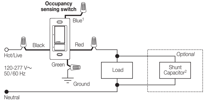
Wiring Diagram 13 Single Location Installation with Shunt Capacitor 1, 2, 3 -OPS6M-DV and -VPS6M-DV
