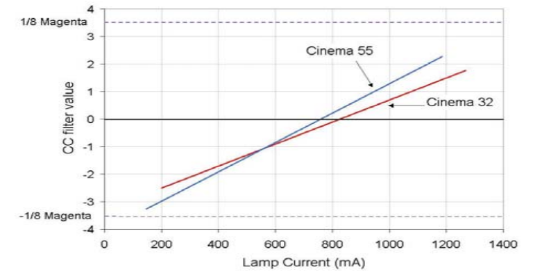
Color vs. Lamp Current for T12HO Cinema Lamps (Chart 3)
