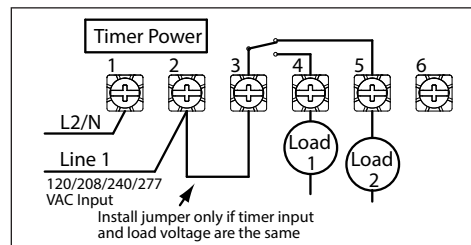
ET1115 configured for SPDT load switching
