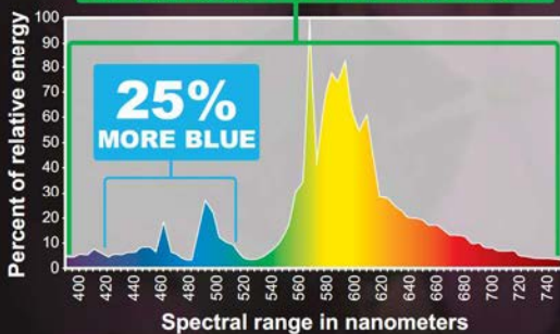
Spectral Distribution for EYE LU1000B/HTL/EN
