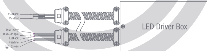
LED DRIVER BOX WIRING GUIDE
