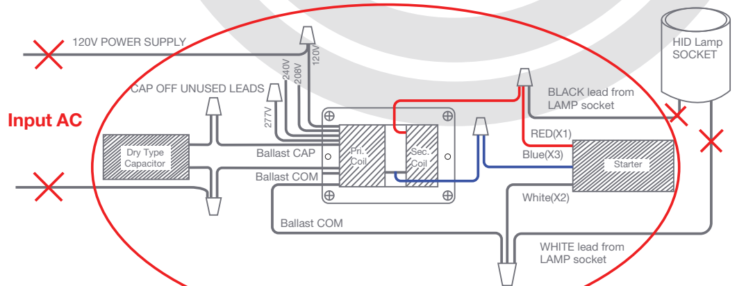
Diagram 2 – Ballast fixture wiring modification
