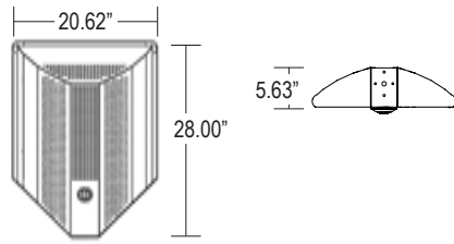
Dimensions for 3 & 4 Brick Unit
