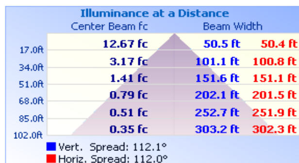
Lux Distance Curve
