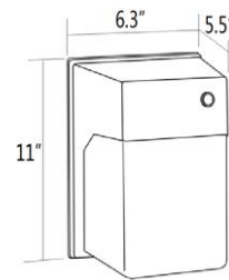
W=6.30" D=5.5" H=11"
