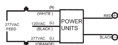
277V TAP CONNECTION
