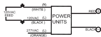
120V TAP CONNECTION
