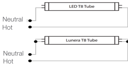
Correct Wiring
