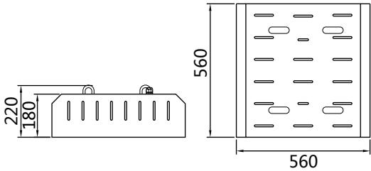
Hook/Chain Mount
