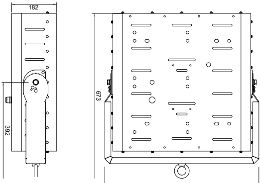
Hook Mount
