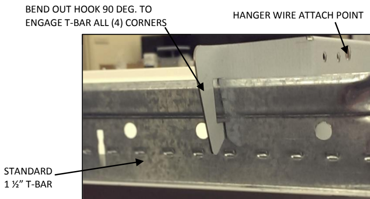
Figure 1: Built In T-Bar Clip
