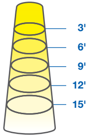
8.5MR16DIM/930SP15
