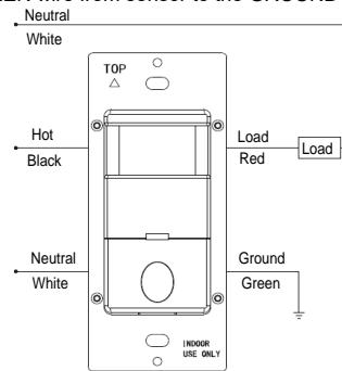
Wiring Diagram
