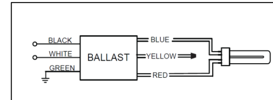
Retrofit with One Lamp
