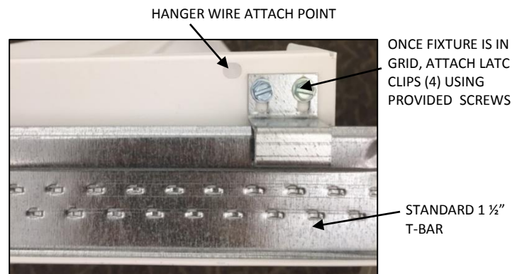
Figure 2: LATC Installation (ORDERABLE OPTION)
