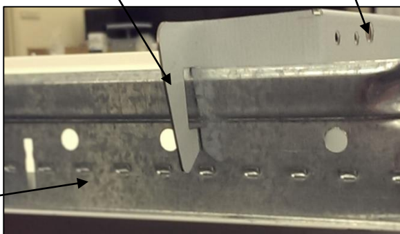
Figure 1: Built In T-Bar Clip
