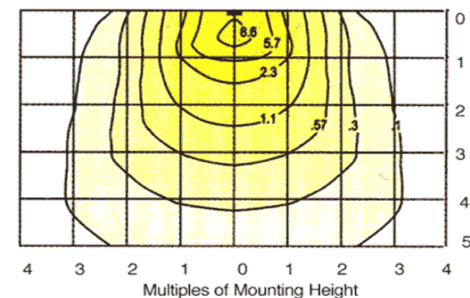
250w HPS @ 16' Mounting Height
