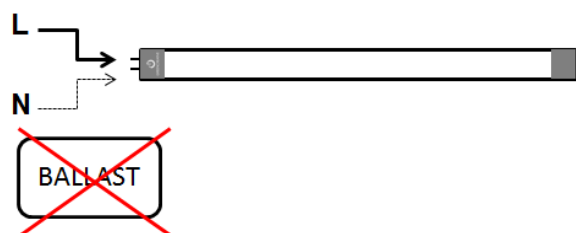
Diagram 3 – Single tube wiring
