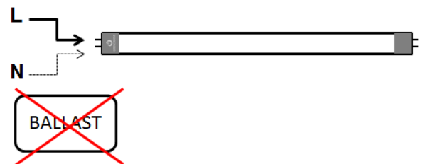
Diagram 3 – Single tube wiring
