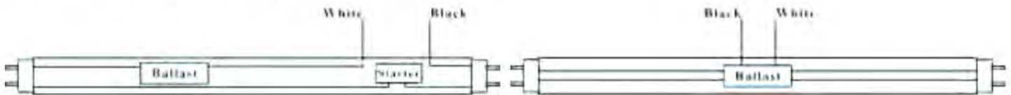
Inductive ballast type
