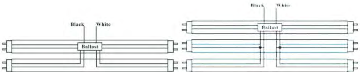
Ballast with 2 lamps
