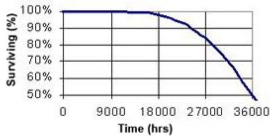
[Graphs_Lumen Maintenance]
