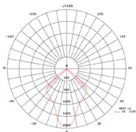
50° Beam Angle
