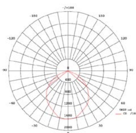
100° Beam Angle
