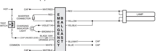
FIG 109aBH ONE (1) 36 W - 55 W LAMP WITHOUT AC BALLAST
