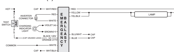
FIG 109BH ONE (1) 14 W - 55 W LAMP WITHOUT AC BALLAST
