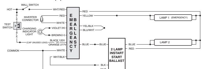
FIG 104BH TWO (2) LAMP INSTANT START BALLAST
