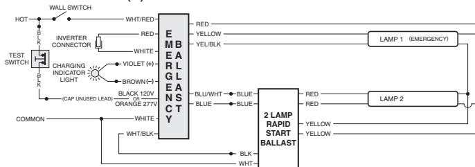
FIG 124BH TWO (2) LAMP RAPID START BALLAST
