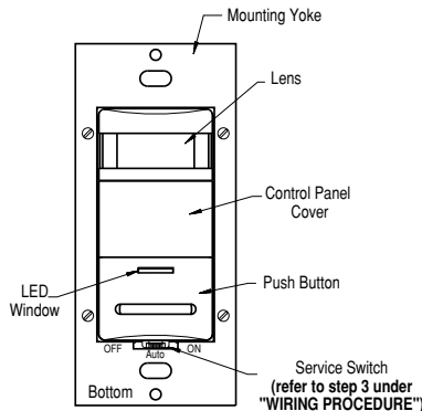
Figure 2 - Sensor Features
