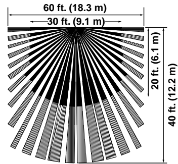
Figure 1 - Field-of-View (Horizontal)
