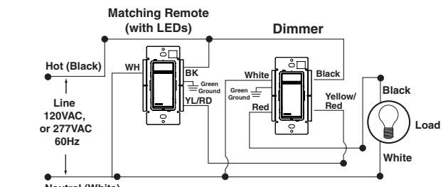
Dimmers VPE04 VPE06 VPX10 VPX12-7L Fan Speed Control VPF01 Switch VPS15 Matching Dimmer Remotes VP00R-1L VP00R-7L Matching Switch Remote VPOSr-1L NOTES: 1) VPS15, VPOSr-1L and VP00R-1L have screw terminals, VPE04, VPE06, VPX10, VPF01, VPX12-7L and VP00R-7L have leads
