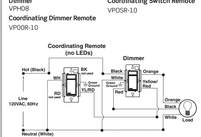
Dimmer VPH08 Coordinating Dimmer Remote VP00R-10 Coordinating Switch Remote VPOSr-10 NOTES: 1) Coordinating remote VP00R-10 and VPOSr-10 have screw terminals, VPH08 has leads 2) Black and Red terminals on coordinating remote are unused
