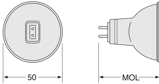
GU5.3
