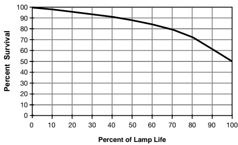
Typical Mortality Curve
