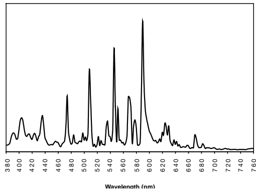
Typical Spectral Power Distribution
