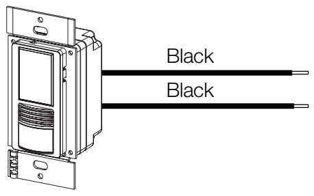
Sensor switch
