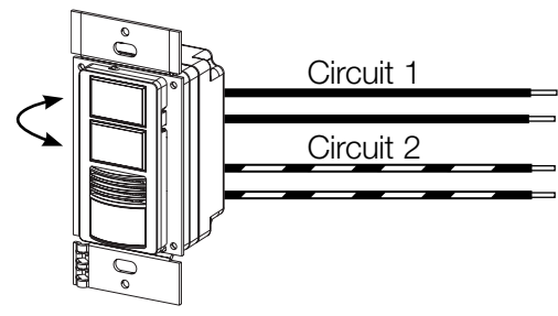
Dual-circuit sensor switch
