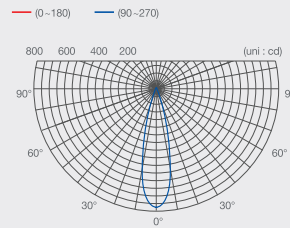
Light Distribution
