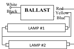
Instant Start T8 Ballast
