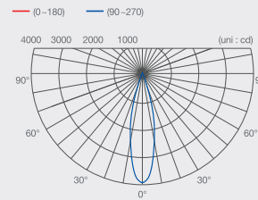
Light Distribution
