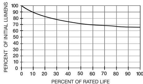
Typical Lumen aintenance Curve
