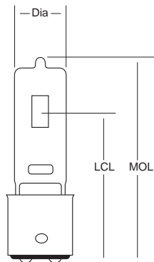
BA15d Base
