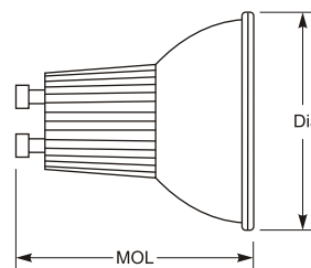
GU10 Base
