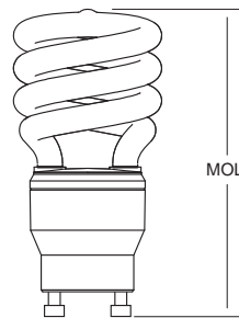
GU24 Base
