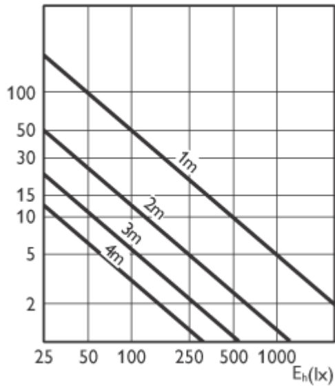
CDM-i 25W/830 25D
