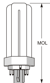
4-Pin Base
