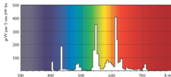
PL-C/830
